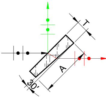
NOTE: Mark beamsplitter surface with a arrow on the side
